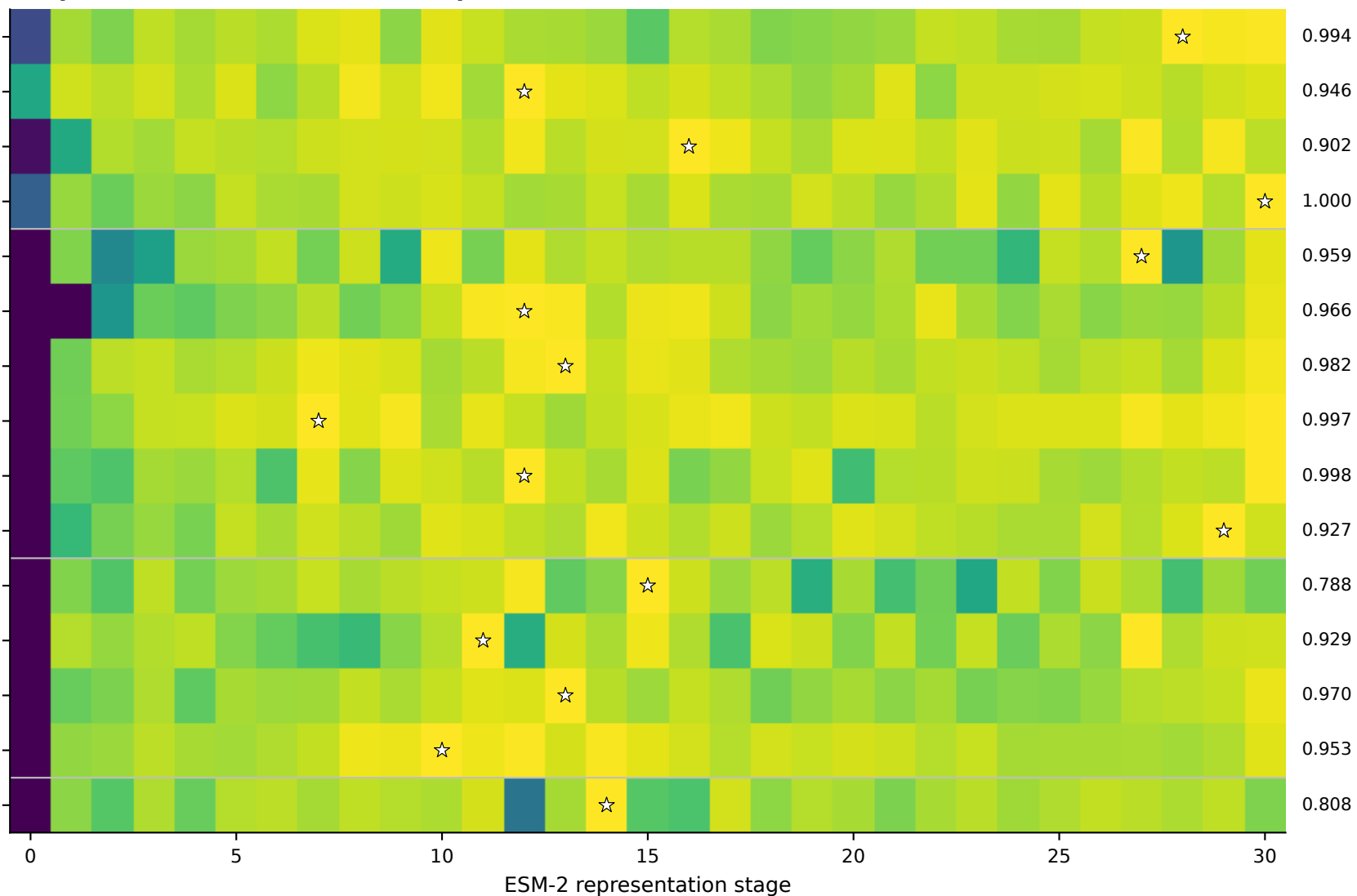
B Epistatic information transit map
